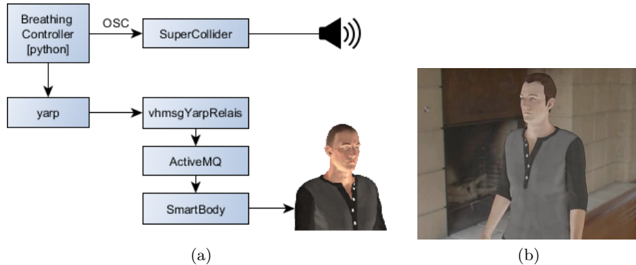
Fig. 5: (a) Software architecture of the speech breathing control system (b) Screen capture of the virtual character controlled and rendered using the SmartBody system [1]
